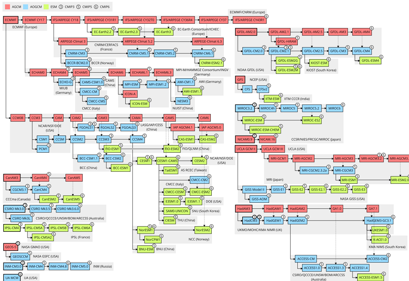
Figure 2. Model code genealogy of participating in the Coupled Model Intercomparison Project (CMIP) phase 3, 5, and 6, including their common ancestor models. Models are distinguished by their complexity into atmosphere general circulation models (AGCMs), atmosphere-ocean GCMs (AOGCMs), and Earth system models (ESMs), indicated by color. Horizontal arrows indicate inheritance between multiple versions of the same model. Vertical solid arrows indicate inheritance between different models. Vertical dotted arrows indicate inheritance from an AGCM to an AOGCM or ESM (this can also mean that the model is used as a component of the more complex model). The gray shaded boxes indicate an institute and the main country or region where the development was conducted. Numbers in circles indicate the CMIP phase. Model boxes with a thick outline indicate the oldest model of the model family. The genealogy only traces models necessary for placing the CMIP models in the graph and omits versions not included in CMIP. The genealogy was reconstructed based on available literature, CMIP metadata, and online resources. Table S1 contains source data corresponding to this figure including literature references for the model relations.
